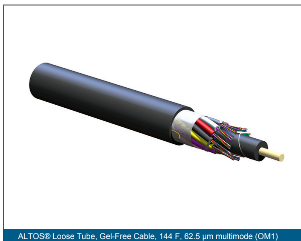
ALTOS® Loose Tube, Gel-Free Cable, 144 F, 62.5 \mu m multimode (OM1)
