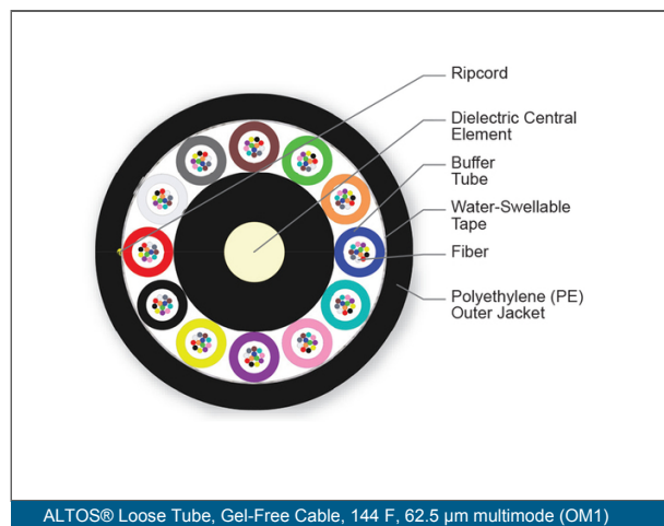
ALTOS® Loose Tube, Gel-Free Cable, 144 F, 62.5 \mu m multimode (OM1)
